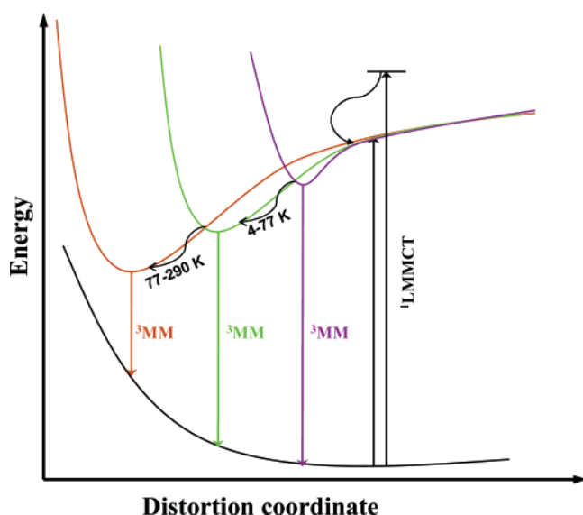
Figure 6. Qualitative description of the photophysical processes in \text{Au}_3 . The same principles are valid for \text{Ag}_3 and \text{Cu}_3 , for which two instead of three {}^3\text{MM} emitting states are involved.
