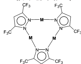
Chart 1. Structure of {[3,5-(CF 3 ) 2 Pz]M} 3 Complexes (M 3 )
